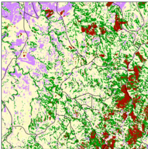
SUPERVISED CLASSIFICATION OF LANDSAT 5 IMAGE (02.06.2007) Analysis by the authors.
